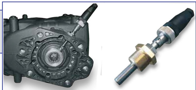
ZRPM1 RPM Counter Inductive proximity sensor, c/w female connector M12 4 pin, IP67, field attachable, ring nut reduction M18 x 1. Power Supply: 12/24 VDC
